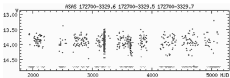
ASAS V-band light curve of V730 Sco. Note the heightened period of activity around HJD+3200 that suggests a non-periodic phenomenon.
