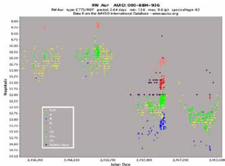
Figure 8. AAVSO light curve of the Tauri star RW Aur JD 2456156–2457503 (16 August 2012–25 April 2016). 79 observers contributed 3,175 visual and multicolor observations to this light curve.
